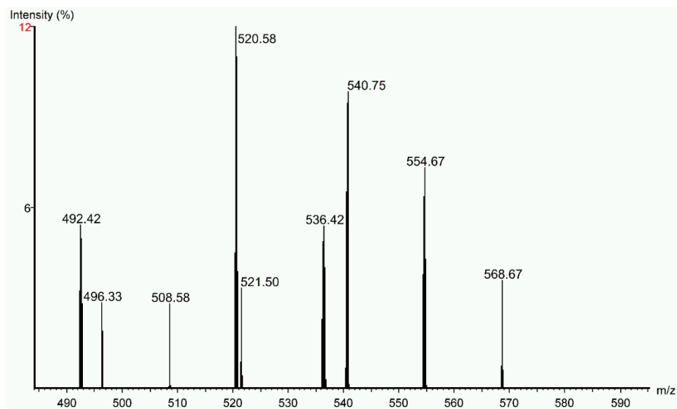
Figure 31. Mass Spectrum of the leaves of Taxus × media (SOTINKY08) showing a taxane at m/z 536 [M + NH_4]^+ .
