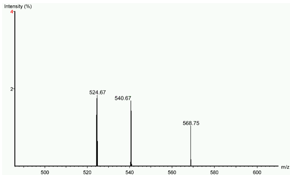
Figure 35. Mass Spectrum of the leaves of Taxus x media (SOTINKY36) showing none of the five taxanes present.
