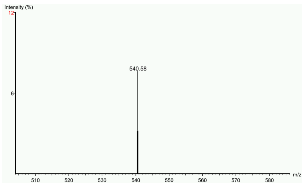
Figure 32. Mass Spectrum of the stem of Taxus × media (SOTINKY08) showing none of the five taxanes present.
