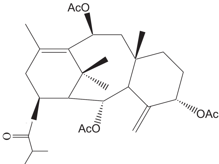
Figure 22. 2 \alpha ,5 \alpha ,10 \beta -triacetoxy-14 \beta -isobutyryloxy-4(20),11-taxadiene. C 30 H 44 O 8 532.66 g·mol -1 . [M + NH 4 ] + with expected m/z of 550.34.
