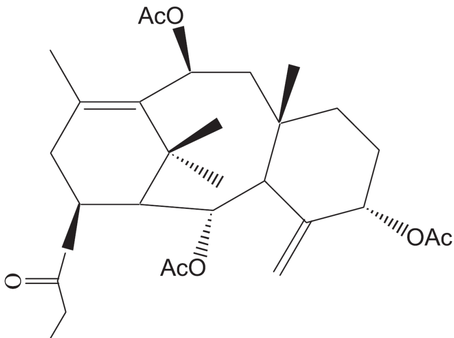
Figure 21. 2 \alpha ,5 \alpha ,10 \beta -triacetoxy-14 \beta -propionyloxy-4(20),11-taxadiene. C_{29}H_{42}O_8 518.61 g·mol -1 . [M + NH_4]^+ with expected m/z of 536.32.
