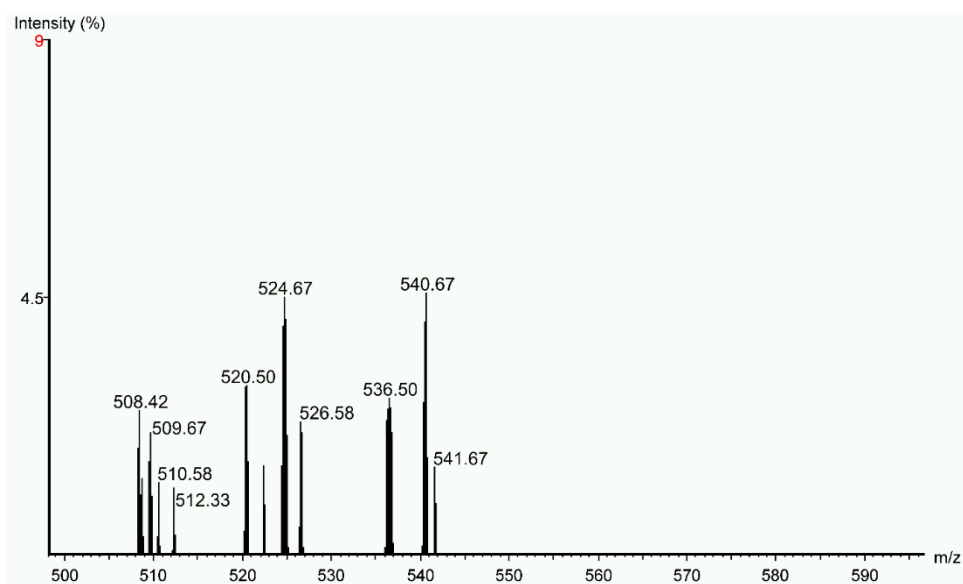
Figure 36. Mass Spectrum of the stem of Taxus x media (SOTINKY36), showing a taxane present at m/z 536 [M + NH_4]^+ .
