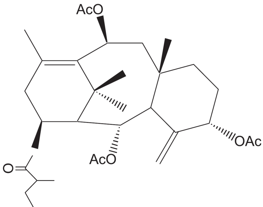
Figure 20. 2 \alpha ,5 \alpha ,10 \beta -triacetoxy-14 \beta -(2-methyl)-butyryloxy-4(20),11-taxadiene. C_{31}H_{46}O_8 546.69 g·mol -1 . [M + NH_4]^+ with expected m/z of 564.36.
